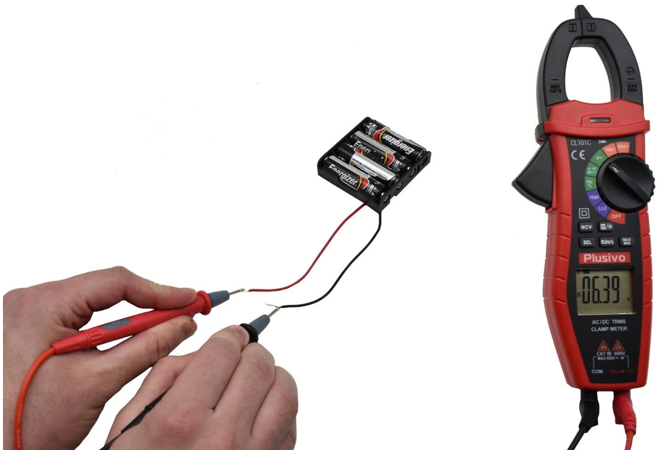
Figure 23. The measured voltage in this figure is 6.39 V DC.
