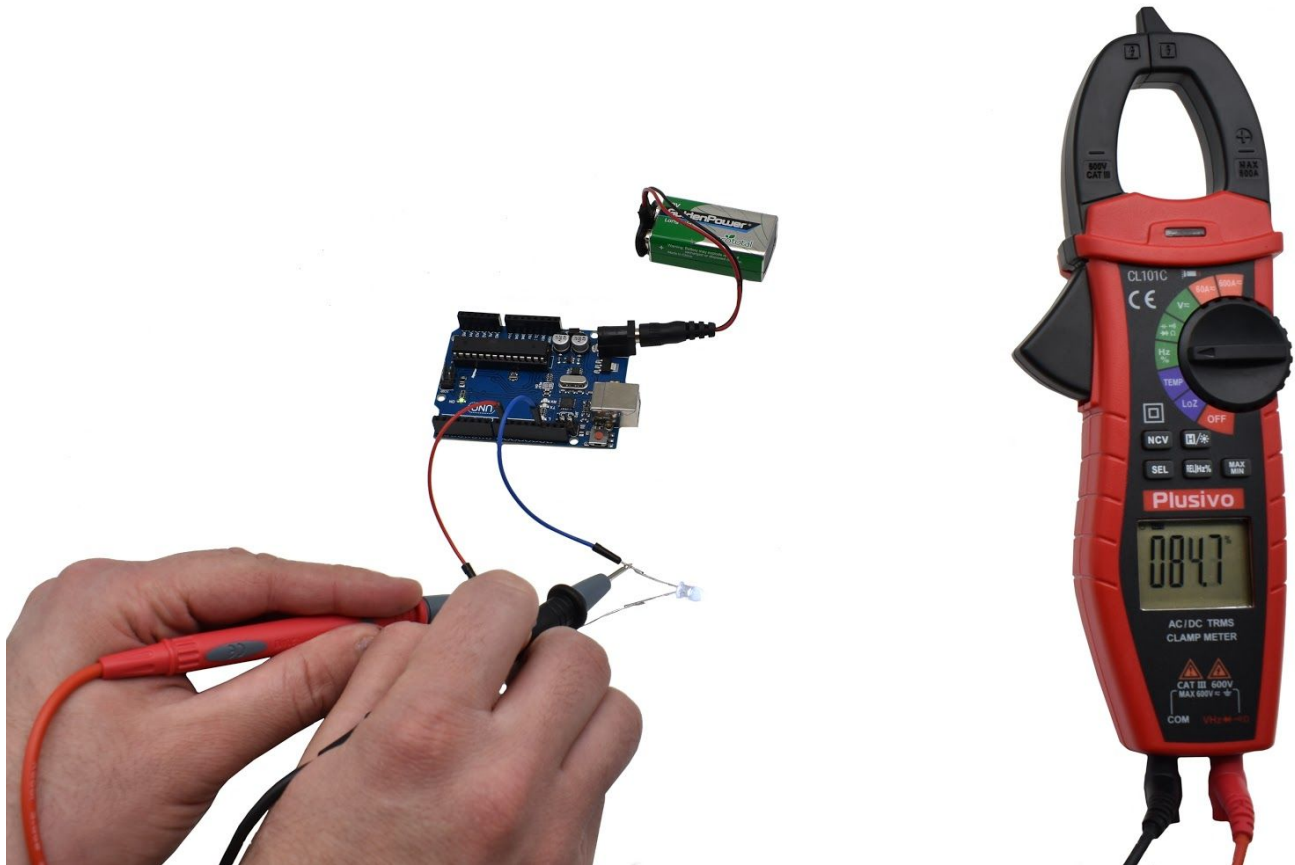
Figure 19. The measured duty cycle in this figure is 84.7 %.
