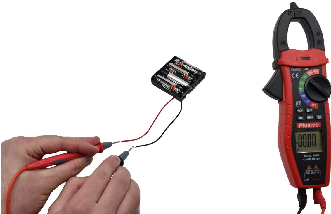
Figure 24. The measured voltage in this figure is 0 V DC.
