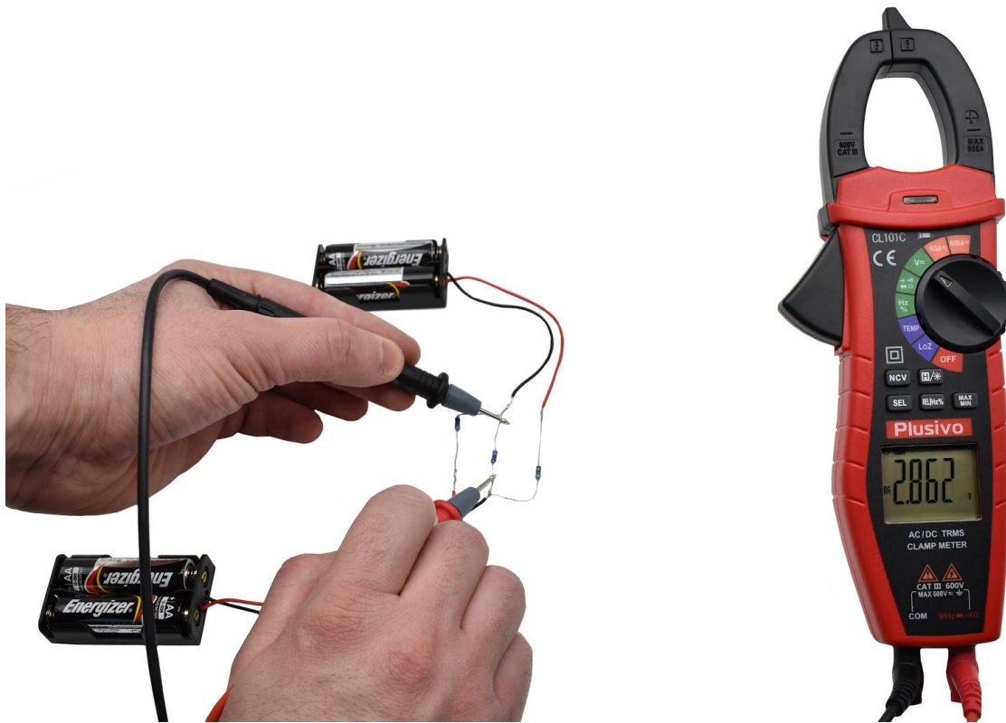
Figure 35. The measured voltage in this figure is 2.862 V DC. The measured voltage around the 47 \Omega resistor is 328.4 mV.
