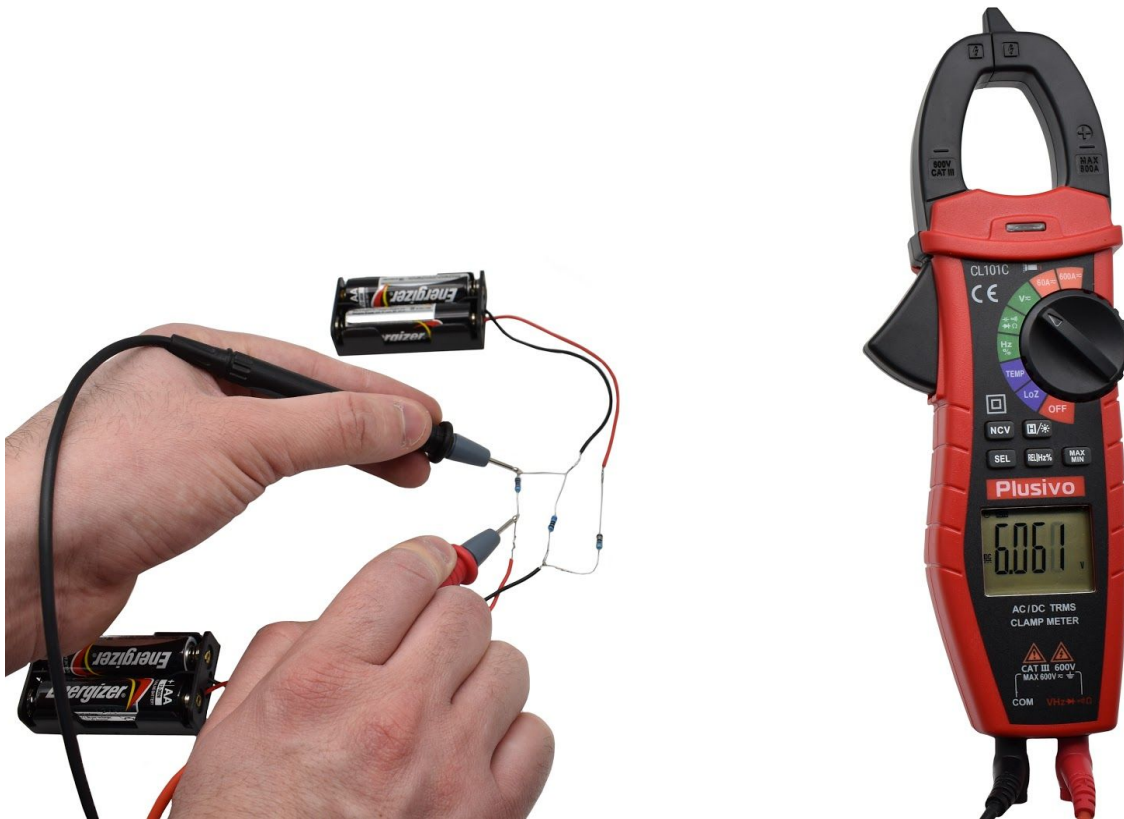
Figure 34. The measured voltage in this figure is 6.061 V DC.
