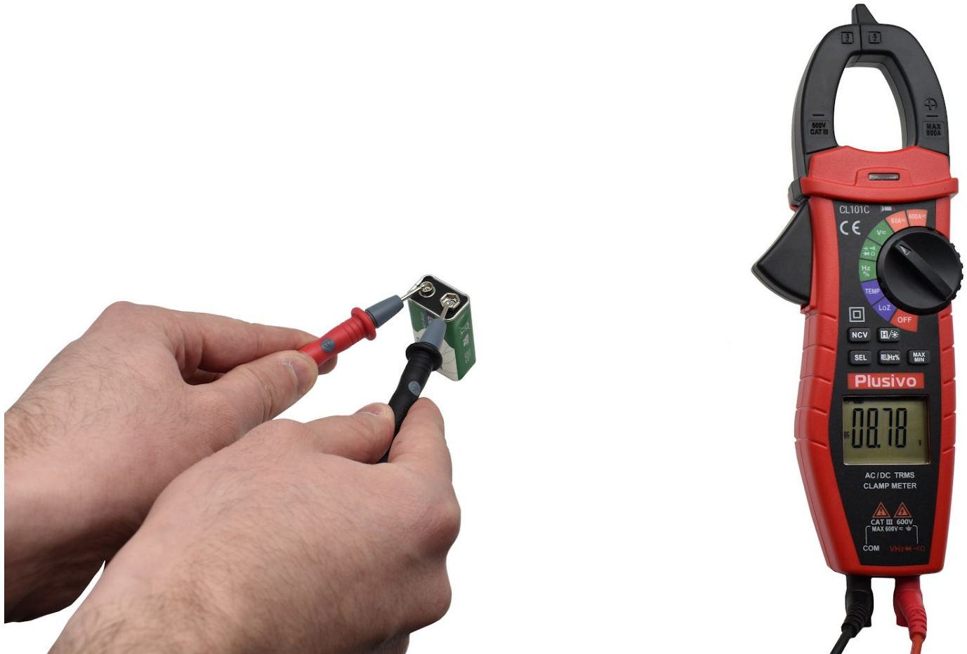
Figure 40. The measured voltage in this figure is 8.78 V DC.
