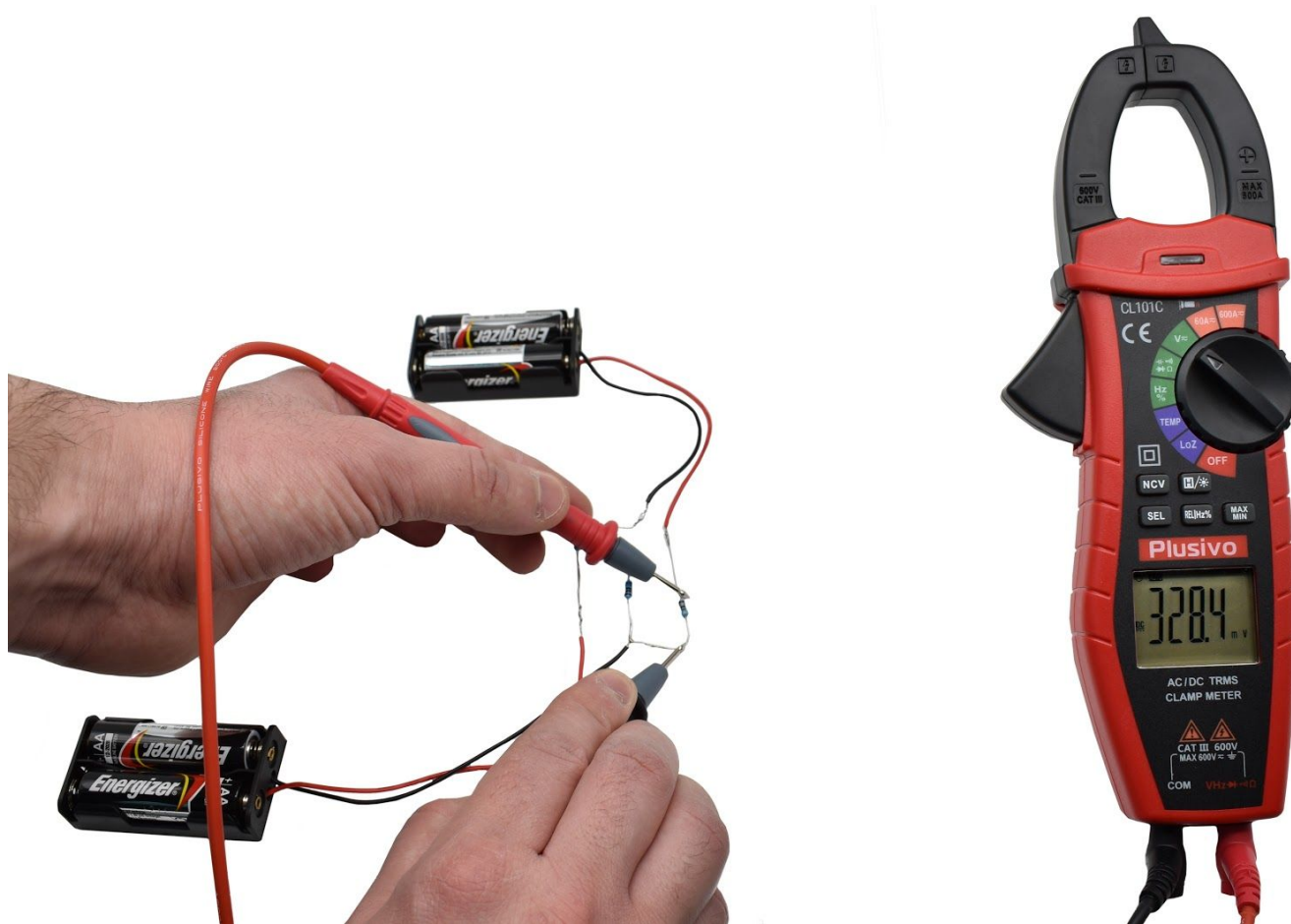
Figure 36. The measured voltage in this figure is 328.4 mV DC.
