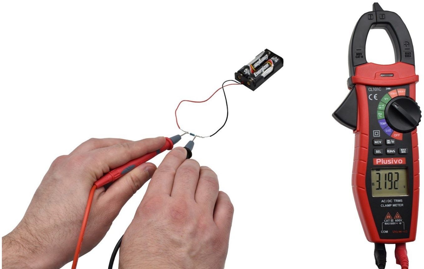
Figure 31. The measured voltage in this figure is 3.192 V DC.
